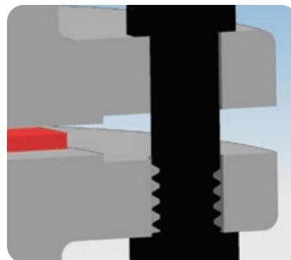
Flat Gaskets
