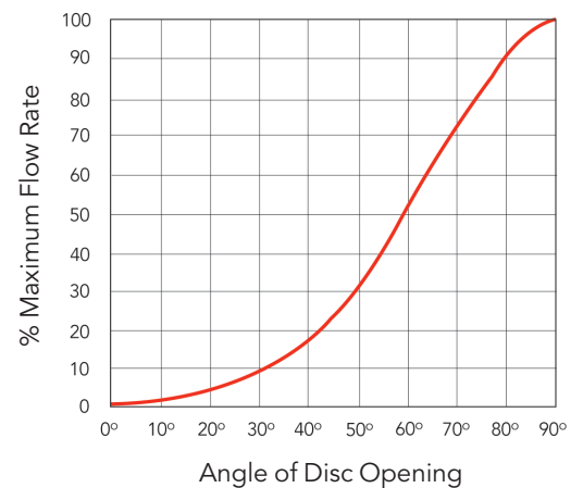
Figure 5: Flow Curve
