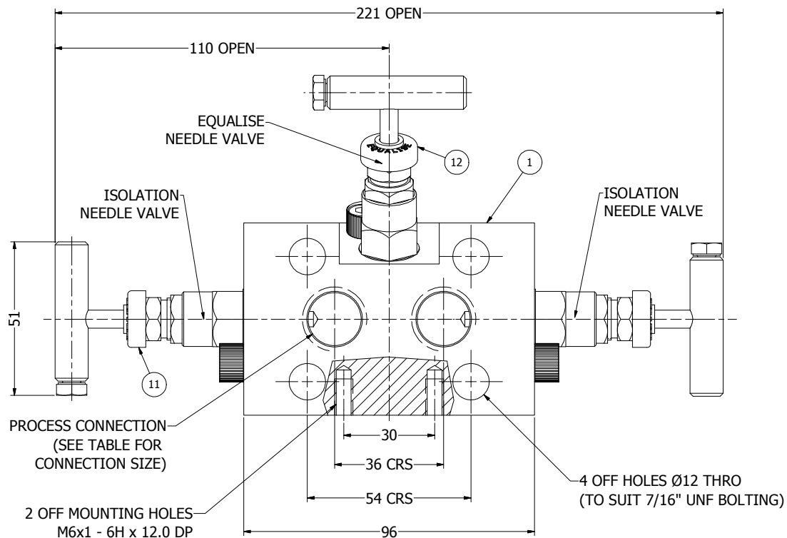
NEEDLE VALVE DETAILS
