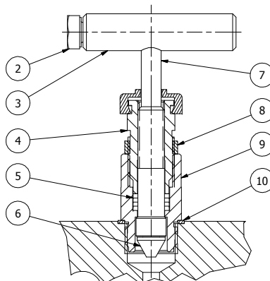
NEEDLE VALVE DETAILS
