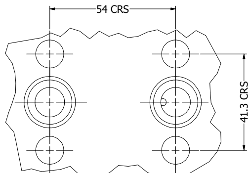
DIRECT MOUNT INSTRUMENT CONNECTION DETAIL A-A
